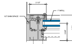
④ VERTICAL JAMB DETAIL 6" = 1'-0"
