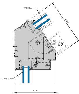
⑤ ADJUSTABLE 35°-60° BAFFLE WITH 6-1/8" GUTTER TRANSITION DETAIL 6" = 1'-0"
