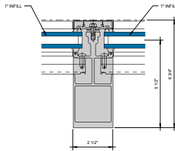
② RAFTER DETAIL 6" = 1'-0"
