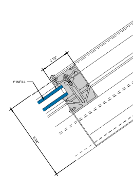
③ HEAD DETAIL 6" = 1'-0"
