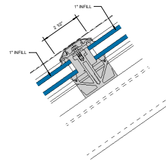
④ PURLIN DETAIL 6" = 1'-0"
