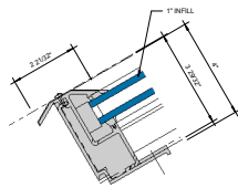
③ APPLIED SILL/TRANSITION DETAIL 6" = 1'-0"
