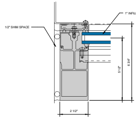
① VERTICAL JAMB 6" = 1'-0"
