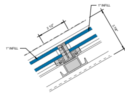
② APPLIED PURLIN DETAIL 6" = 1'-0"
