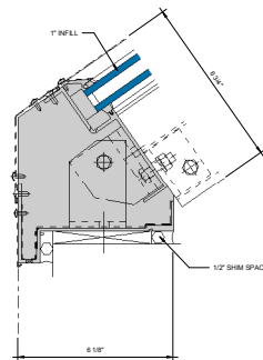
⑥ ADJUSTABLE BAFFLE WITH 6-1/8" GUTTER SILL DETAIL 6" = 1'-0"
