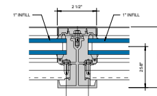
⑤ RAFTER DETAIL 6" = 1'-0"
