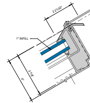
① APPLIED HEAD DETAIL 6" = 1'-0"
